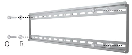
Figure 1 – Attach wall plate to wall.
