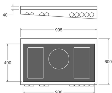
WORKTOP DETAILS
