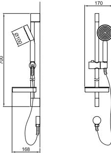
SRA02 Single Function Head on Sliding Rail with Soap Dish
