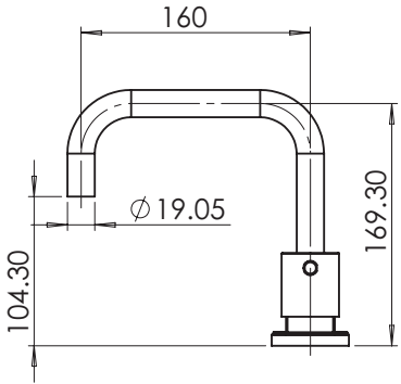
S200S Basin Set Squareneck
