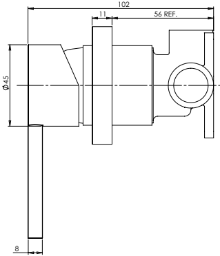
BVSHEXT / BVSHMINT Shower Mixer
