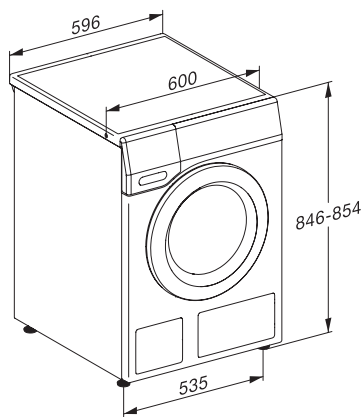
WT1 9/5 kg, drawing, slanted fascia, measures in mm
