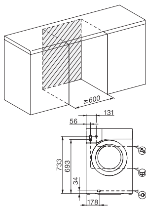
WT1 9/5 kg, installation drawing, slanted fascia or straight fascia, measures in mm
