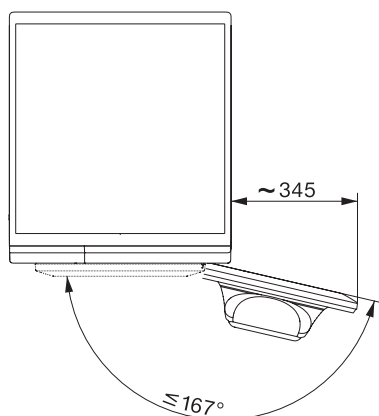
WT1 9/5 kg, drawing, slanted fascia, measures in mm
