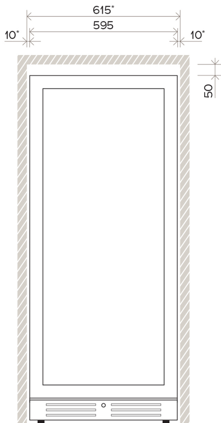
FRONT VIEW
