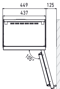
TOP VIEW, HINGE 105°
