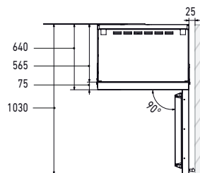
TOP VIEW, HINGE 90°
