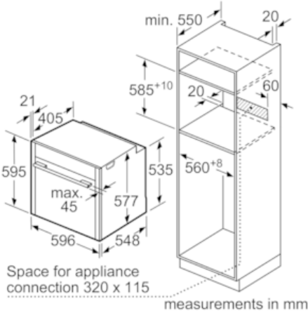
Dimensioned drawings
