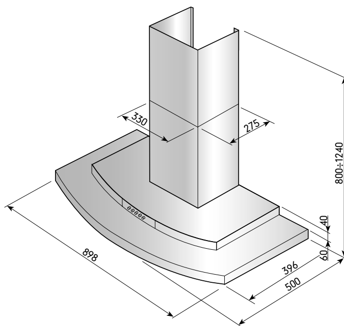
Model B1 Canopy Hood Size: 90cm Extended flue pipe is available from ILVE Power standard Plug in 10 Amp Ducting size: 150mm
