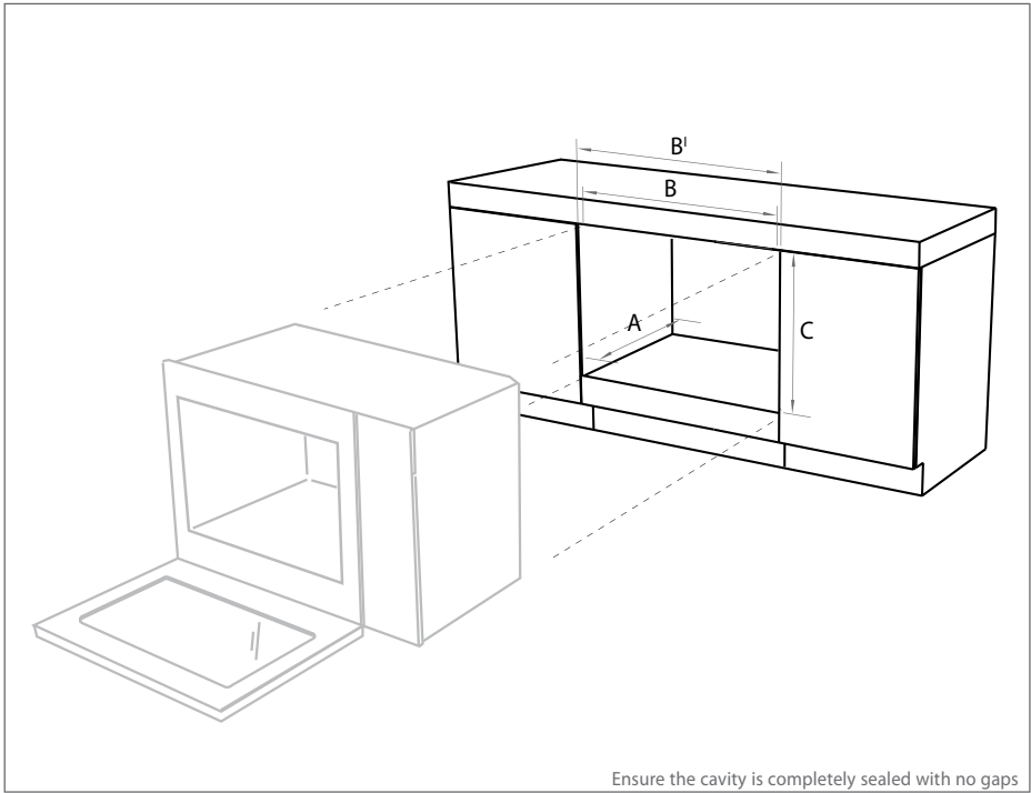
Cabinetry dimensions (mm)
