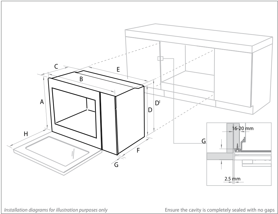
Product dimensions (mm)
