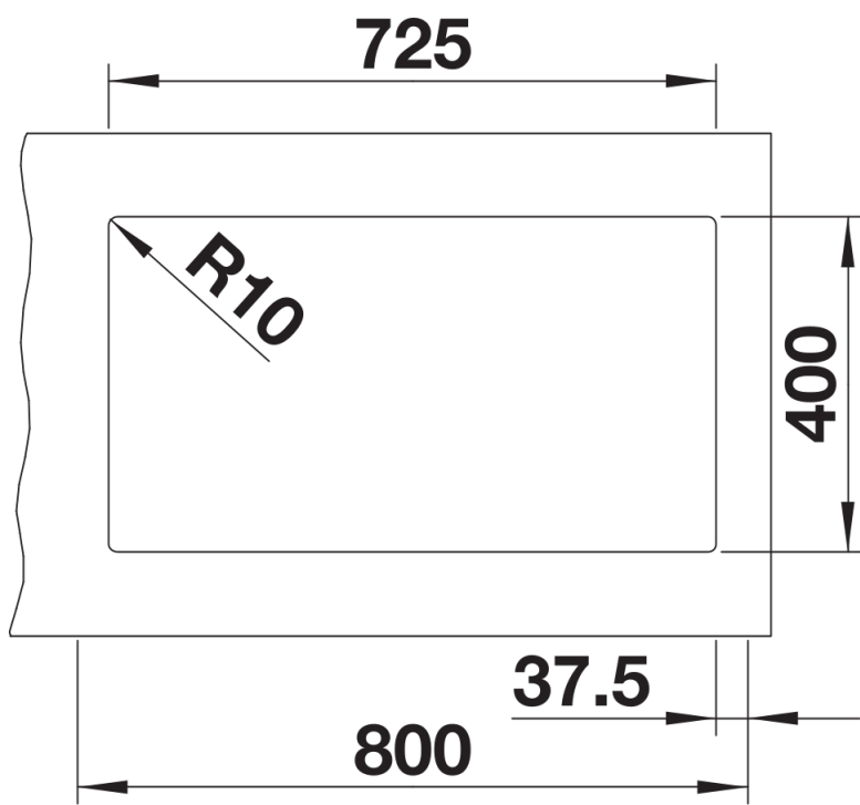
Cut-out
