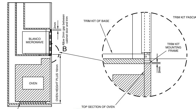
SECTION VIEW
