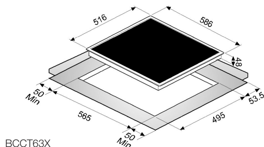
BCCT63X
