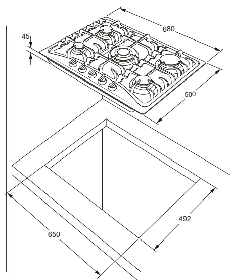
Standard Flushline Installation
