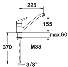
Model BLUNA: Chrome fixed spout
