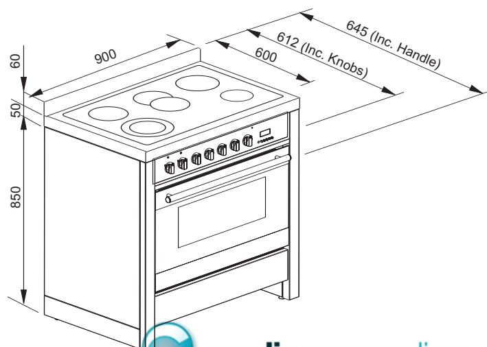
BFS95C
