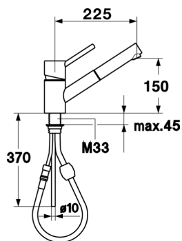
Model BSTYLEP: Chrome pull out spout
