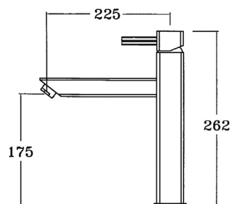
Model BL8301: Chrome fixed spout
