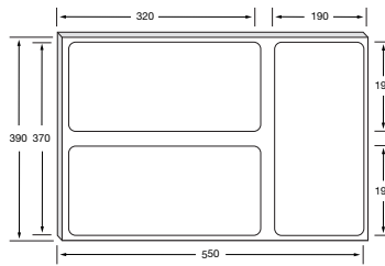
Bin Frame
