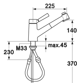
Model BKONOSP: Chrome pull out spout
