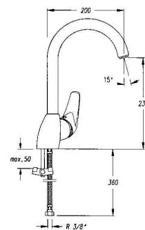
Model B2226: Chrome high arc spout
