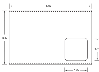
Bin Cover/Adaptor
