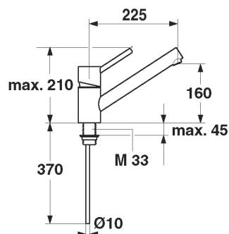
Model BSTYLE: Chrome fixed spout
