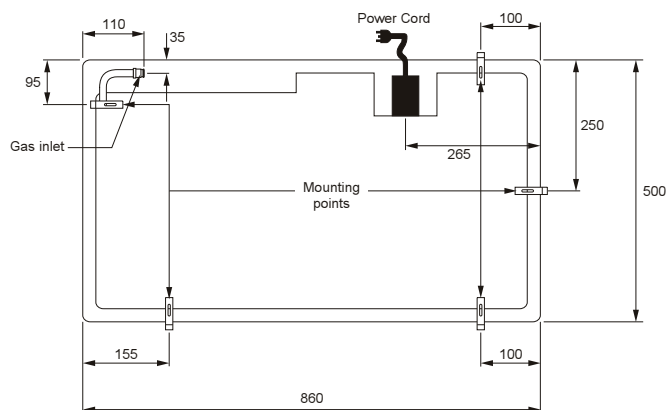
BCG95* 90cm gas cooktop Squareline
