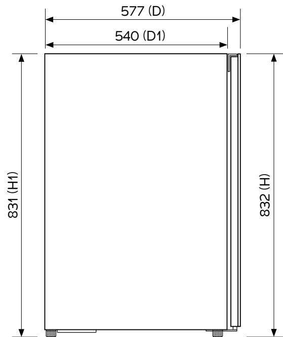
PROFILE VIEW
