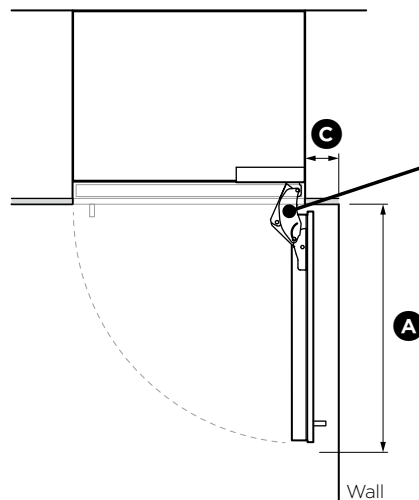
90° DOOR OPENING
