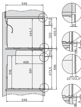
Side view with a H 7000 BP, installation drawings
