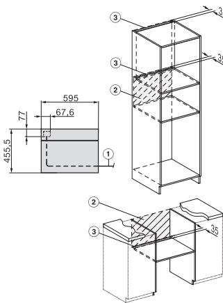
Installation H 7000 BM, installation drawing
