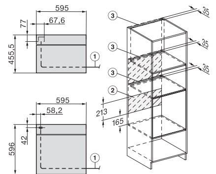
Installation with a H7000 BP, installation drawings
