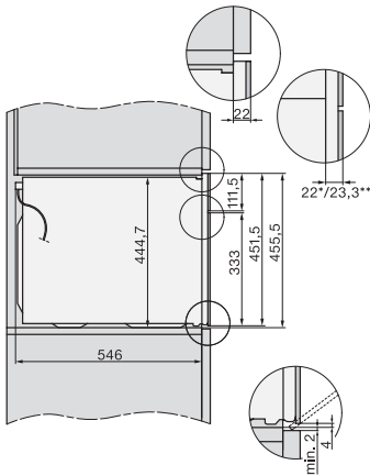
Side view H 7000 BM, installation drawings
