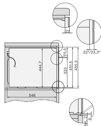
Side view, under bench, installation drawings
