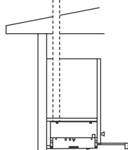
Ducting through roof
