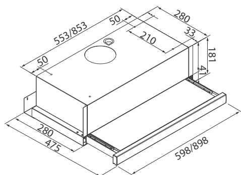
Fig.1 Slideout rangehood
