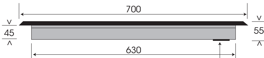
FRONT ELEVATION
