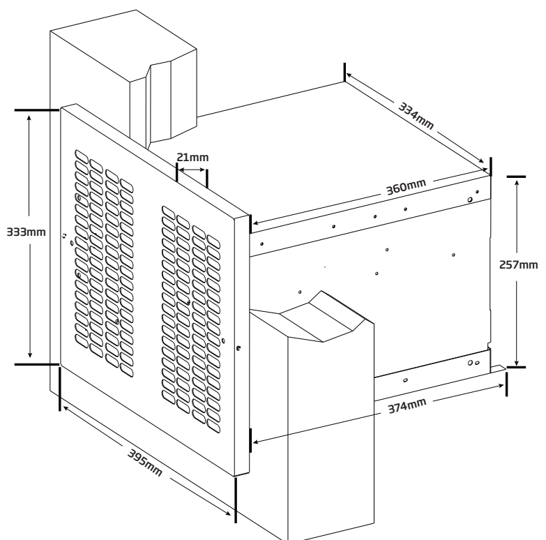
Mounting System
