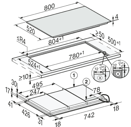
KM 7678-2 FL - (flush installation drawings) 1. Front 2. Mains connection box with mains connection cable, L = 1440 mm 3. Stepped cut-out natural stone worktop 4. Wood support 12 mm (not supplied)
