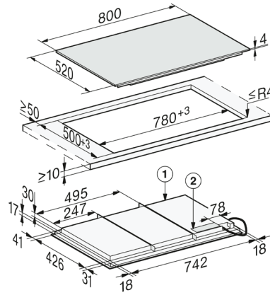
KM 7678-2 FL PowerFlex - (Installation drawing) 1. Front 2. Mains connection box, mains connection cable, L = 1440 mm, supplied loose
