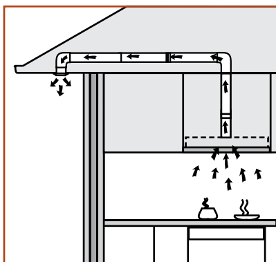
Side Exhaust to atmosphere
