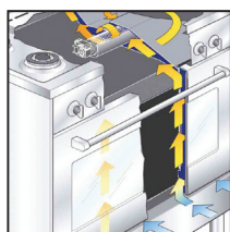
Door and oven cooling
