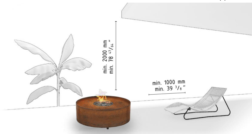
Figure 1: Minimum distance to flammable materials
