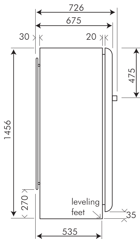
SIDE ELEVATION
