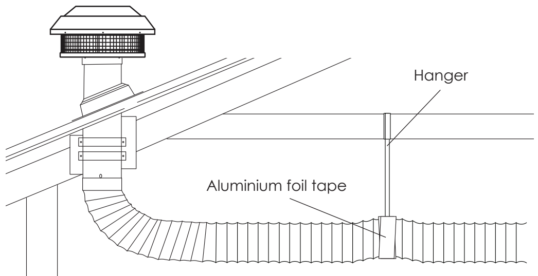
Figure 14 Examples of securing ducting
