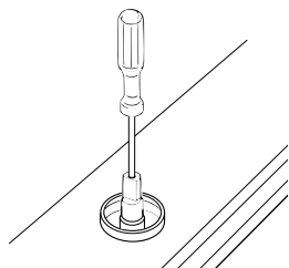
Fig. 9 Minimum burner setting - valves with adjustment screw in the centre of the shaft.
