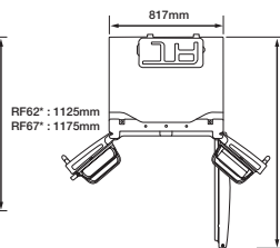
Swing-Type
