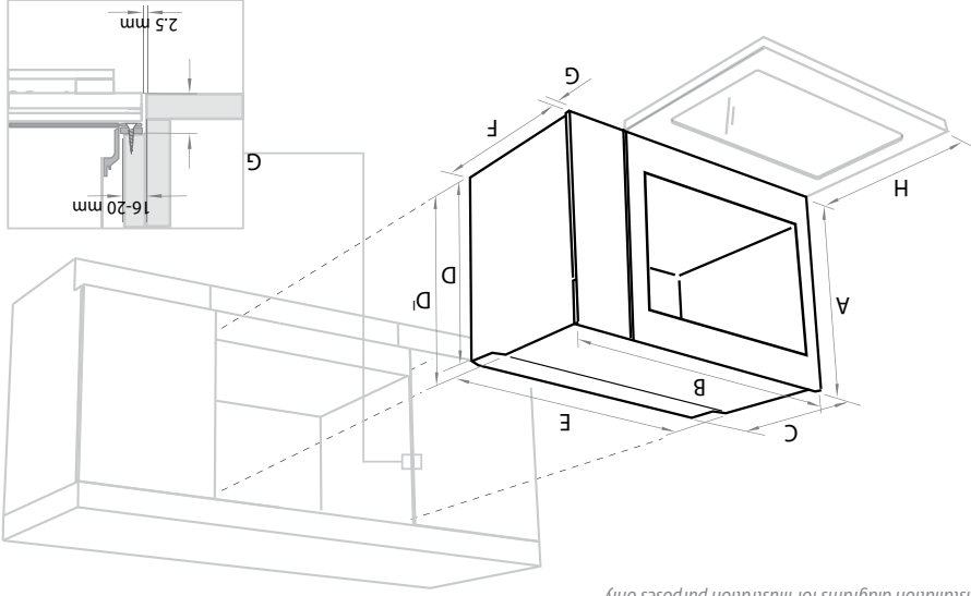
Installation diagrams for illustration purposes only
