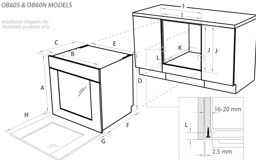
Product dimensions (mm)
