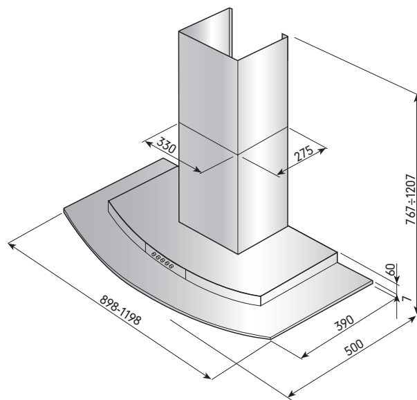
Model: B2 Canopy Hood Size: 90cm and 120cm Power standard: 10 Amp plug Ducting size: 150mm Extended flue pipe is available from ILVE
