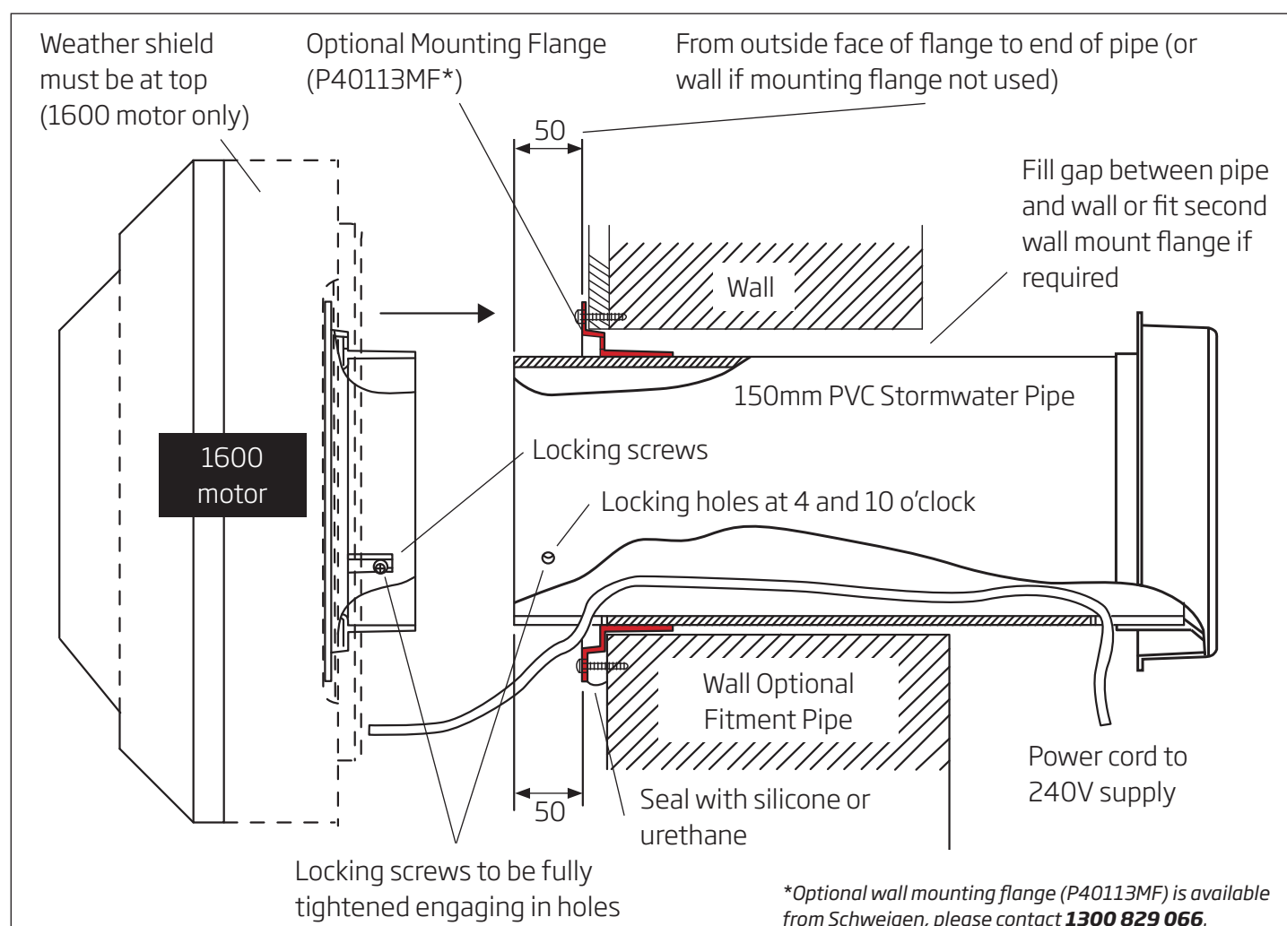
Figure 2 Wall Installation
