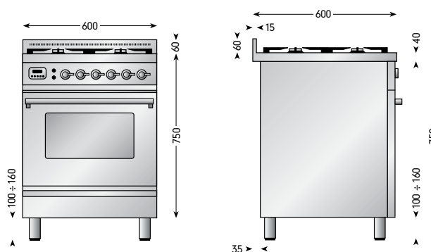
Model PE 60 WMP Total electrical load: 9kW
