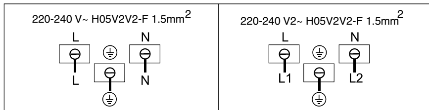
Fig.1 BCCK32N
