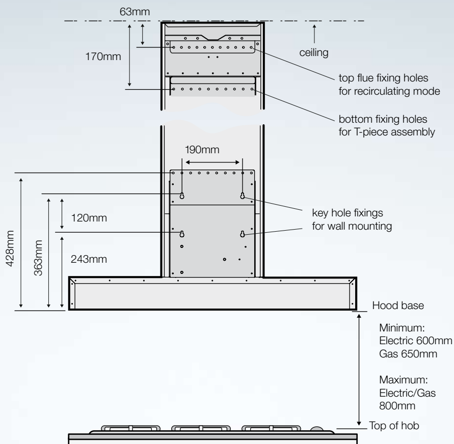
Top Exhaust to atmosphere
