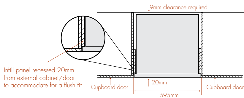
Flush fit (top view)
