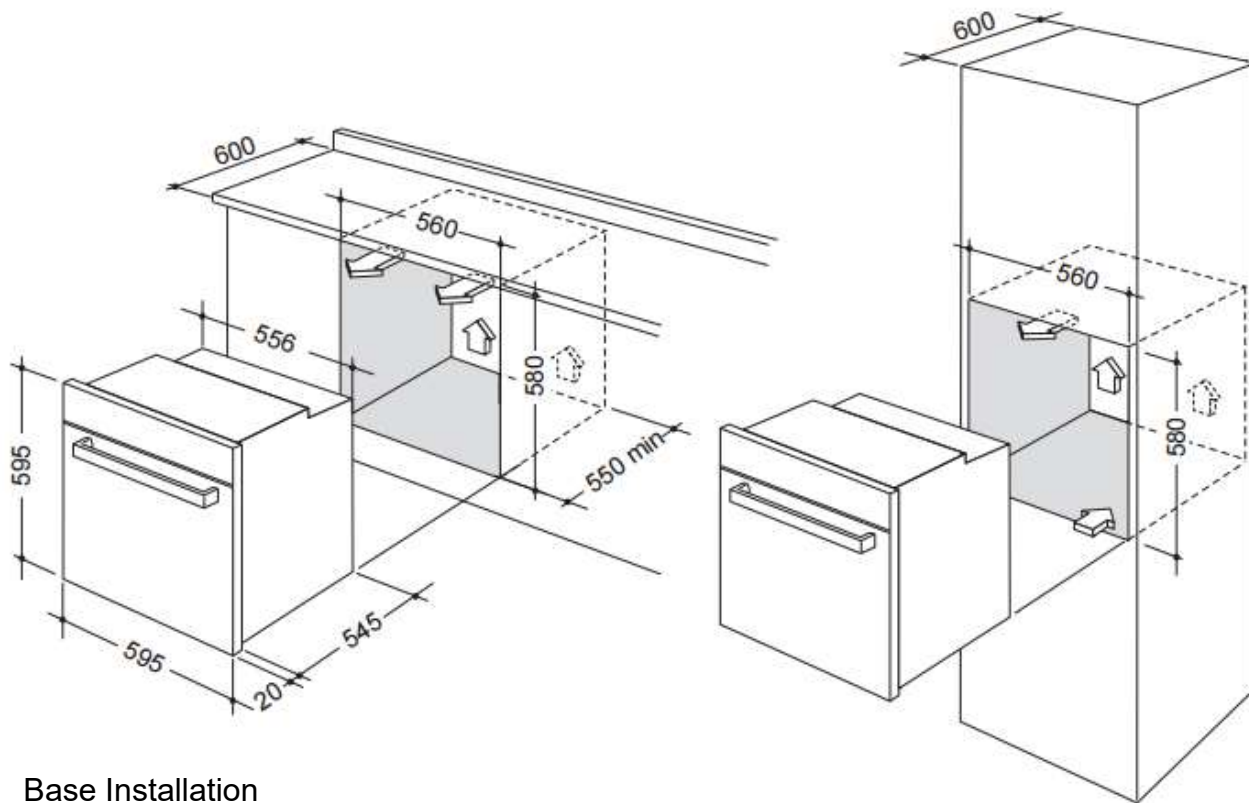
Column Installation
