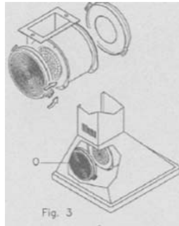
CHANGING THE CARBON FILTER
