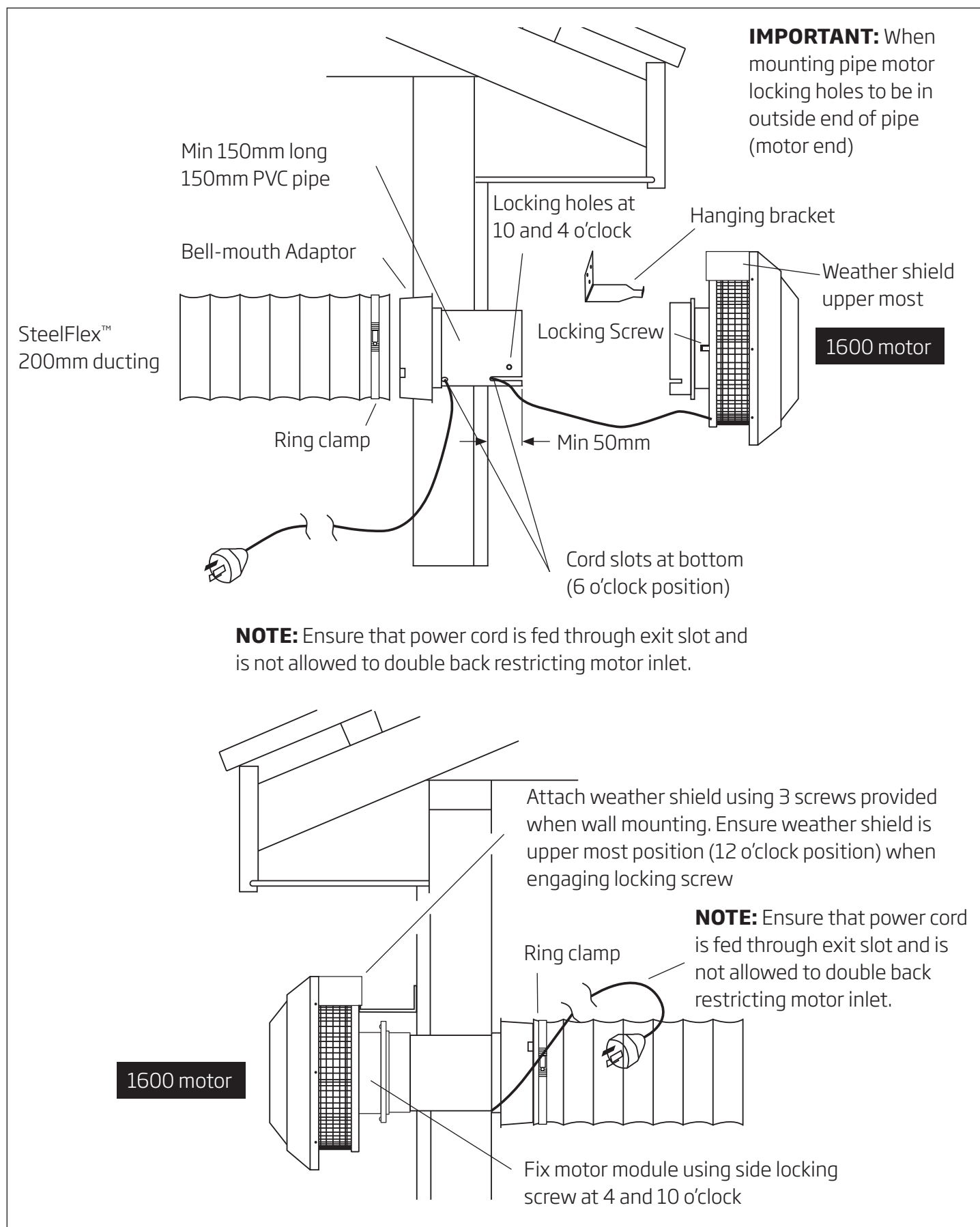
Figure 4: Wall mount option
