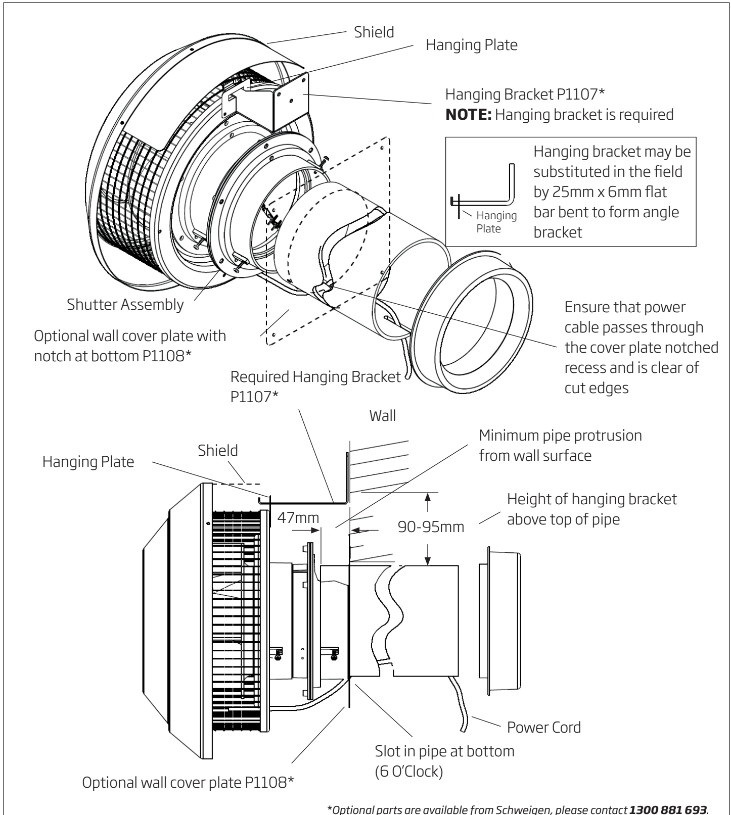
Figure 5: Backdraft shutter wall mount
