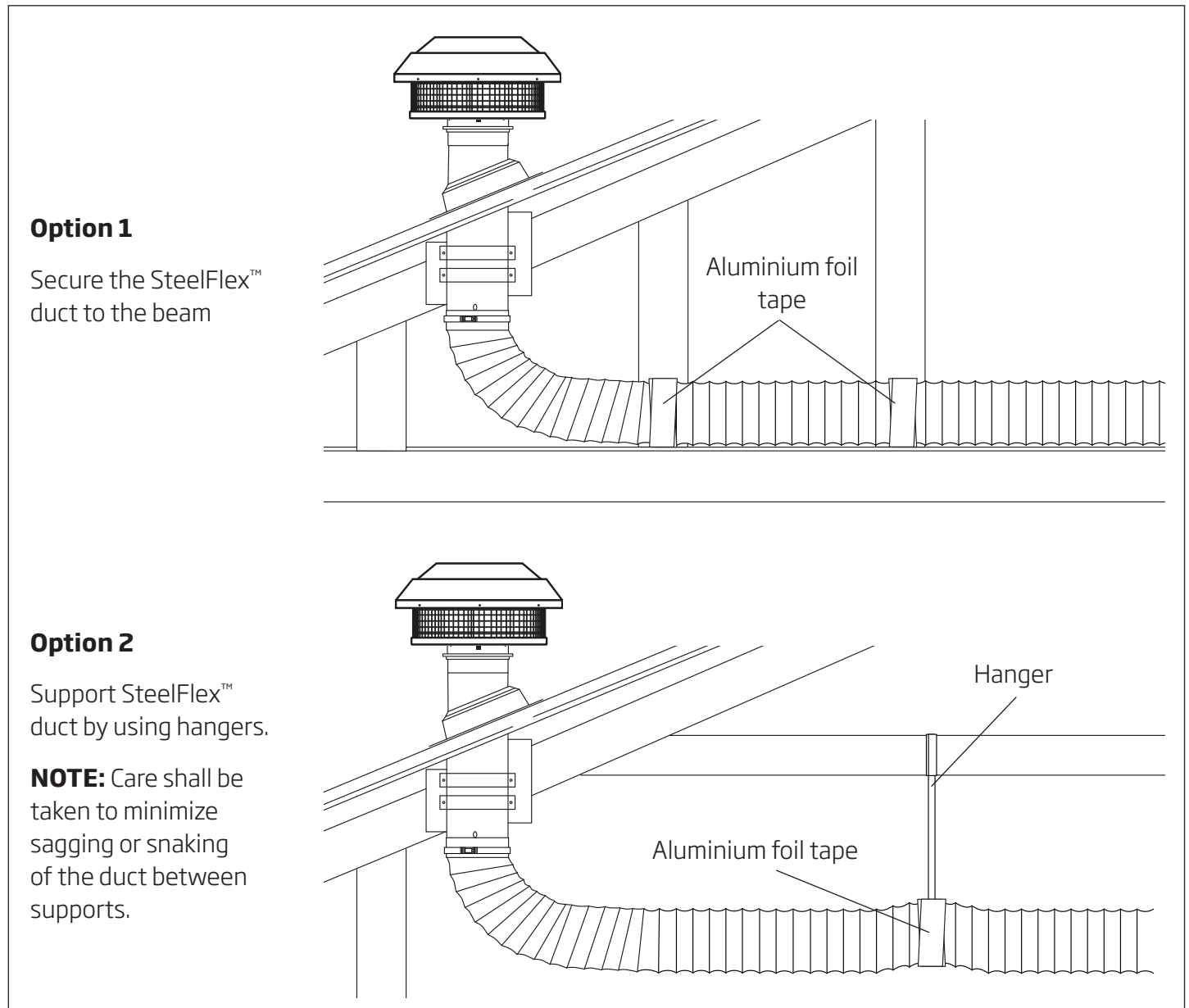
Figure 15: Securing SteelFlex™ Safety Duct
