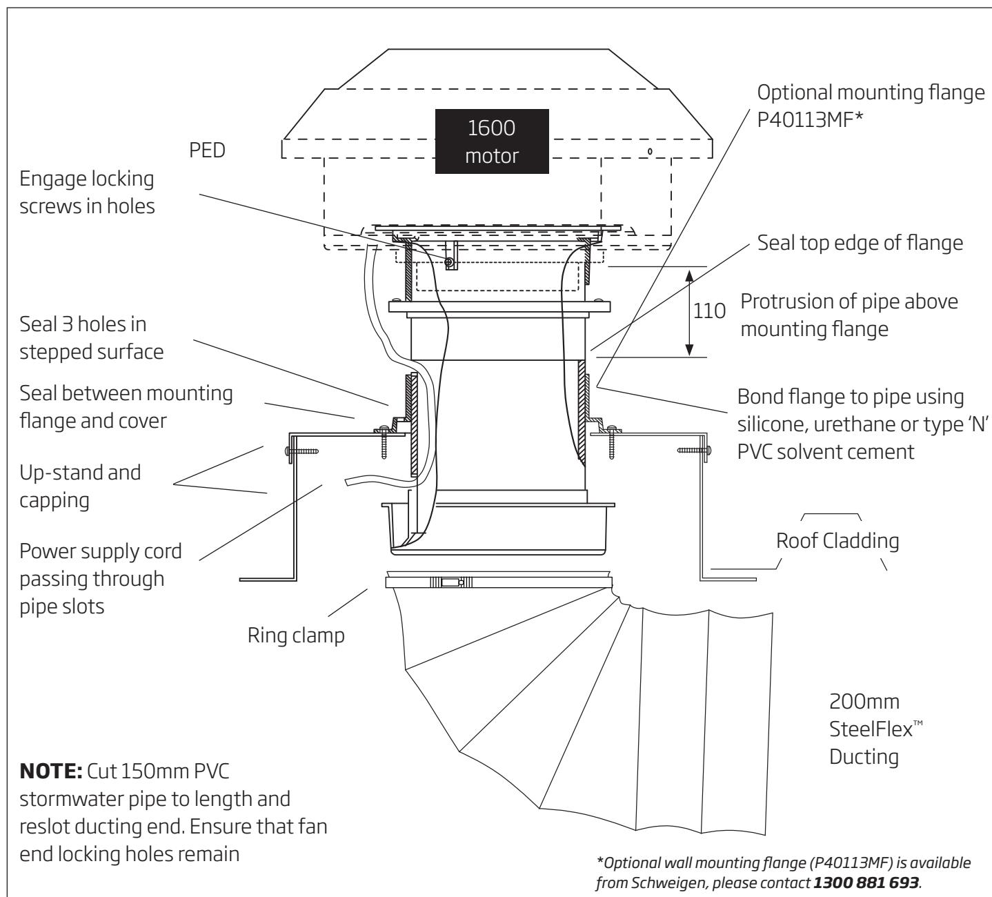
Figure 2: Flat roof installation
