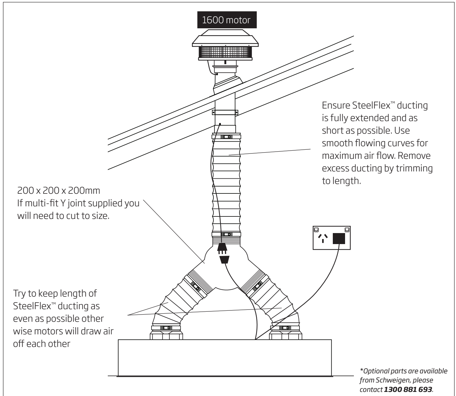
Figure 9: Roof mount option
