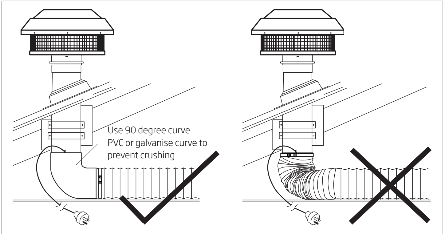
Figure 13: Shallow roof space
