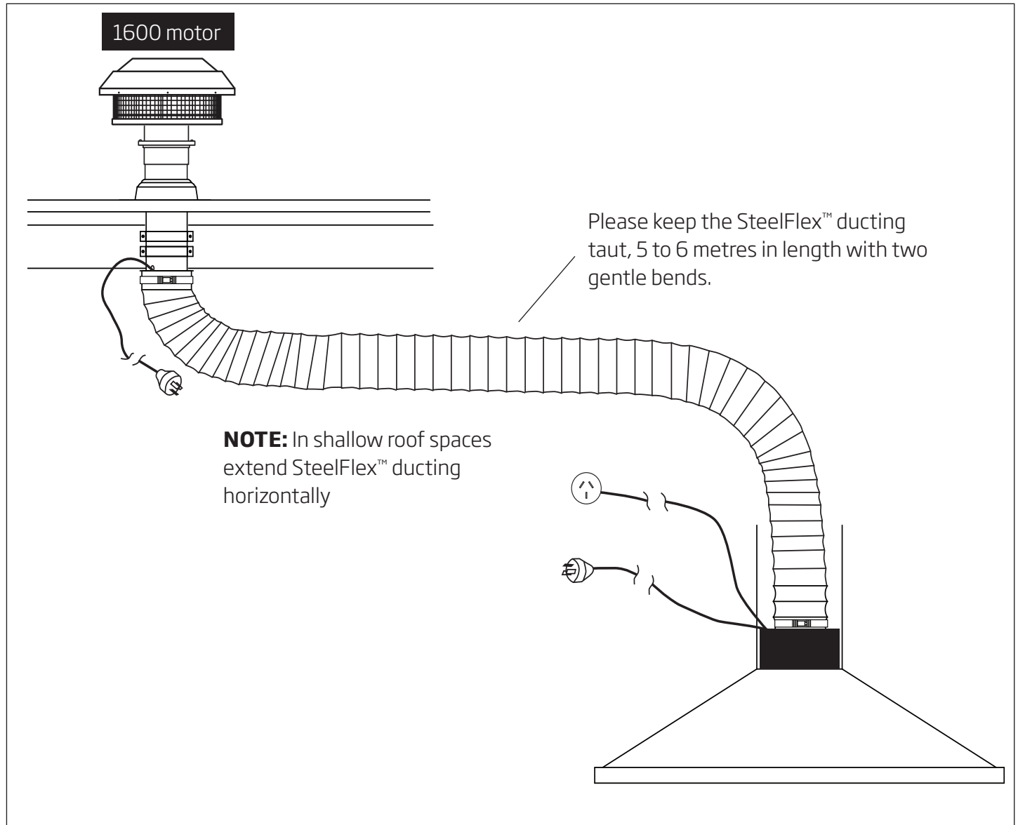
Figure 11: SteelFlex™ Safety Ducting
