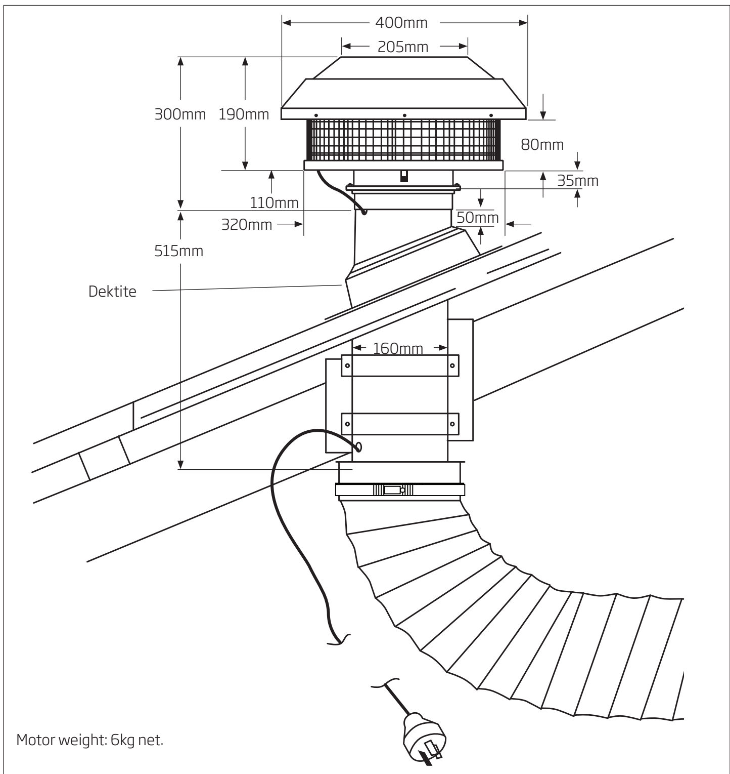
Figure 10: Measurements for Isodrive 1600
