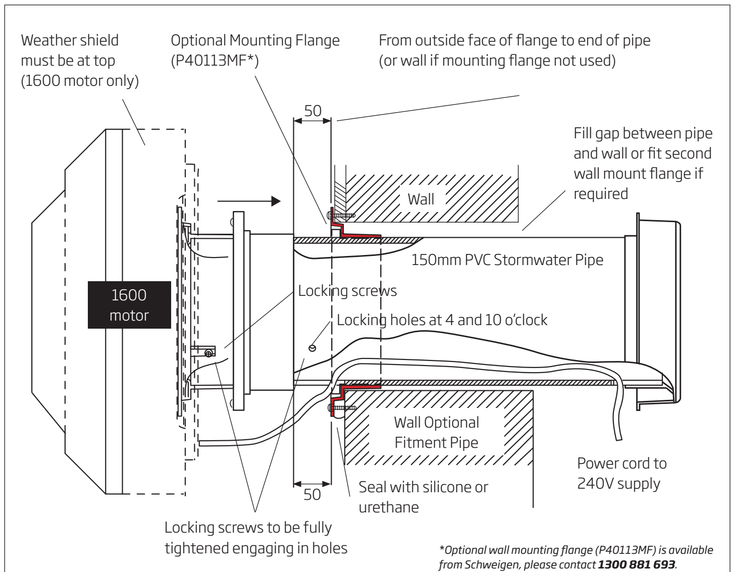
Figure 3: Wall installation
