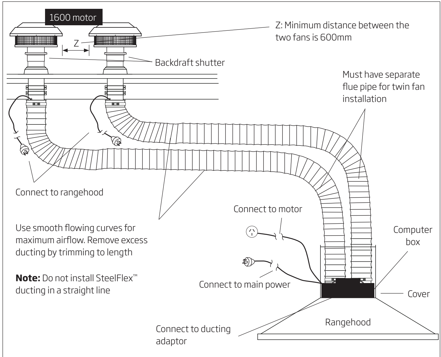
Figure 7: Roof mount option
