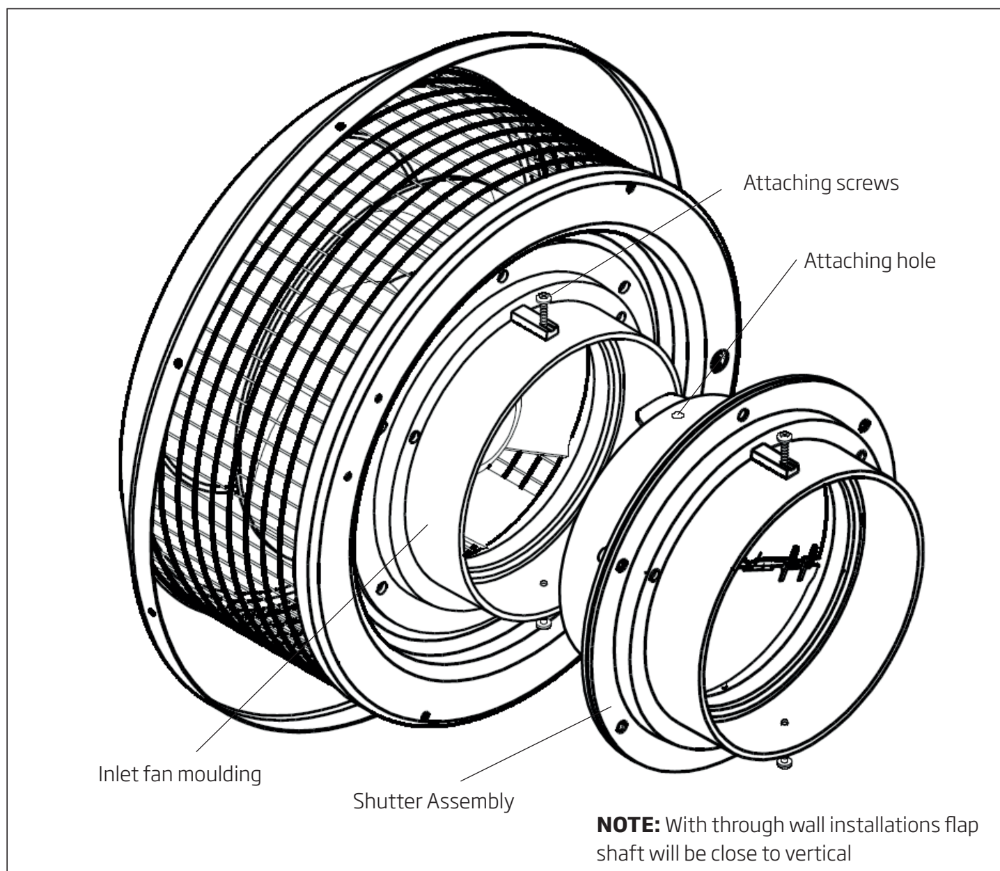
Figure 6: Shutter assembly
