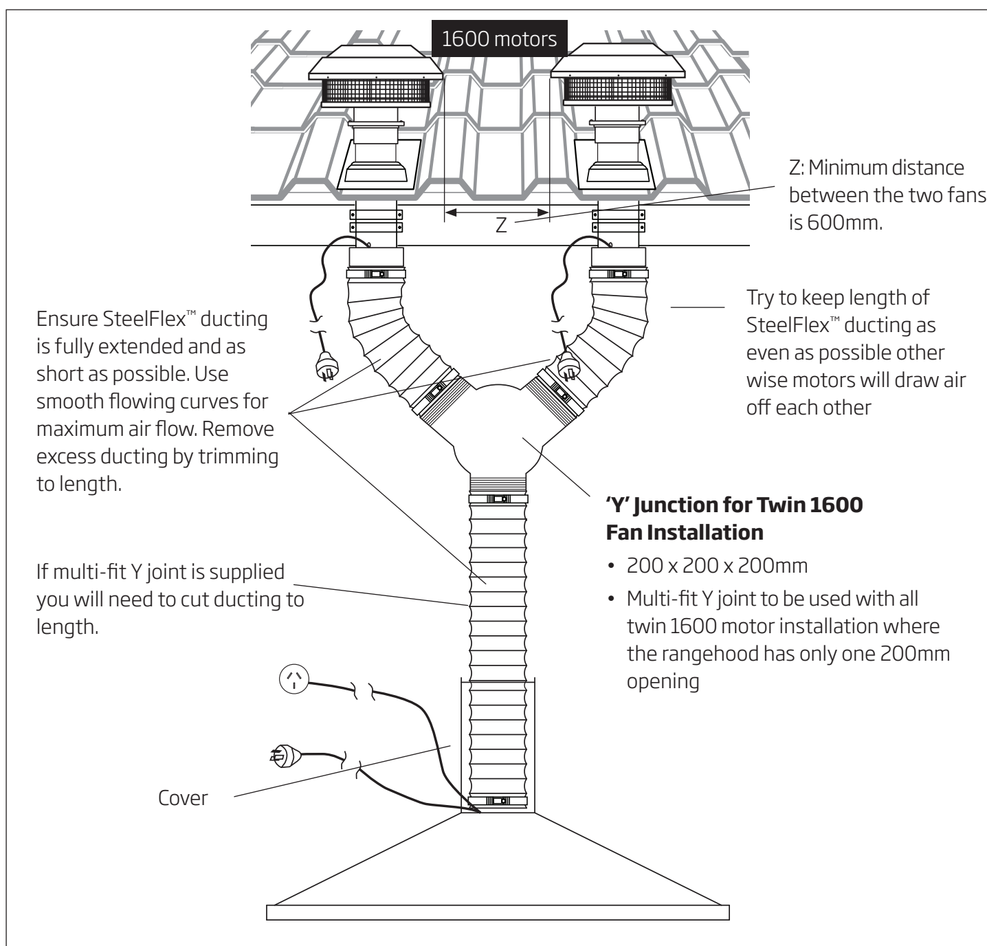
Figure 8: Roof mount option
