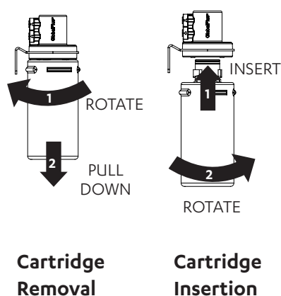
Fig 3. Cartridge replacement
