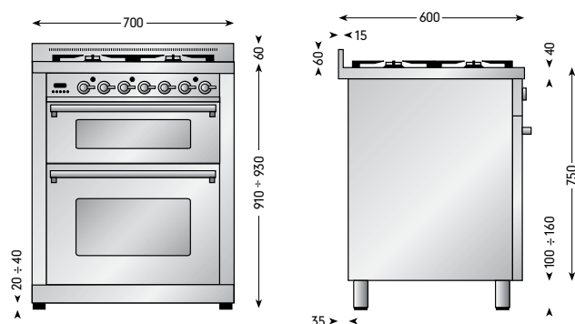
Electric oven Model PD 70 WMP Gas consumption: 40MJ/h Total electrical load: 4.1kW
