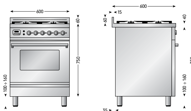
Electric oven Model P 60 WMP Gas consumption: 40MJ/h Total electrical load: 3.7kW
