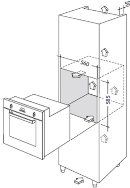
Column Installation
