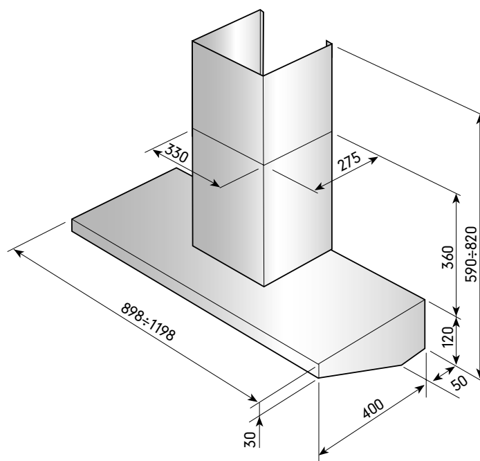
Model: B9 Canopy Hood Size: 90cm Power standard: 10 Amp plug Ducting size: 150mm Extended flue pipe is available from ILVE
