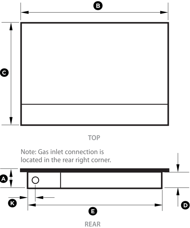
Product and cabinetry dimensions (mm)
