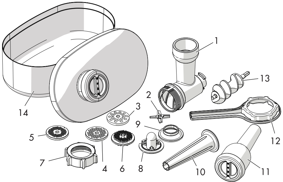
SMMG01 - Multi-food grinder accessory
