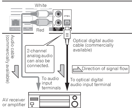
Rear panel
