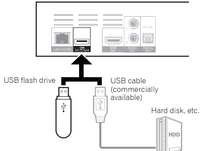
Rear panel
