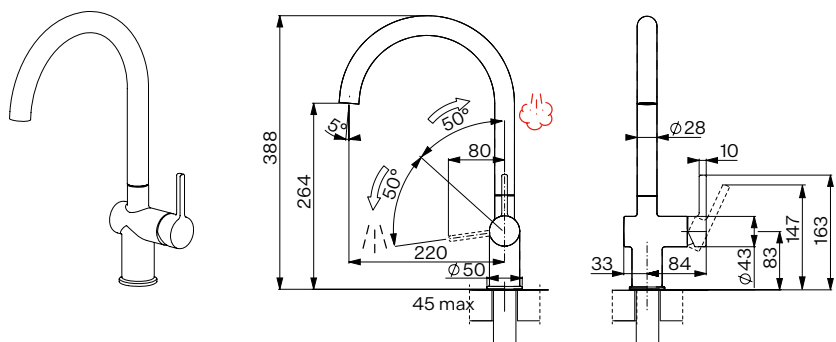
Pull - out L shape 2 jets
