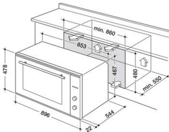
Base Installation
