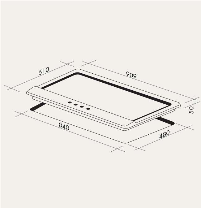
AGH90X | AGH91X AGH90XFFD | AGH91XFFD
