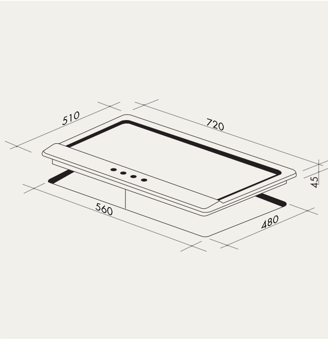
AGH70X | AGH71X AGH70XFFD | AGH71XFFD
