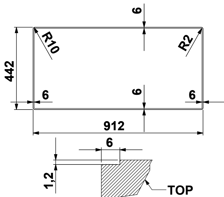
Flush mount Hole
