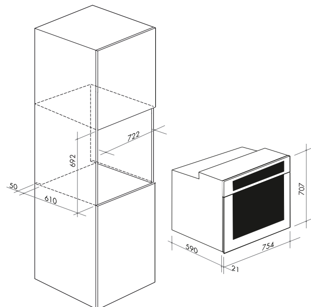
Built-in Oven 76cm Model 760 SPYTCGV Total electrical load: 3.7kw/h
