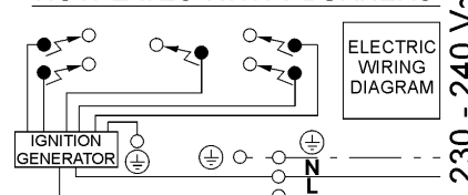
HOTPLATES WITH 5 BURNERS
