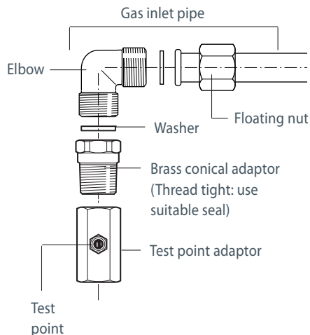
Fig. 6 LPG connection
