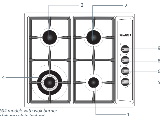
Fig.12a CG604 models with wok burner (no flame failure safety feature)
